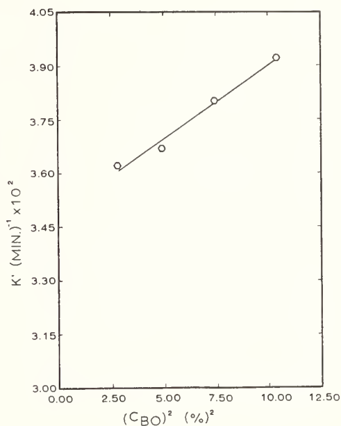
Figure 9. K' versus (C_{BO})^2 : test of a linear relationship between K' and (C_{BO})^2 for waste oil batch #2, CA_0 = 1.495 weight % ASH
